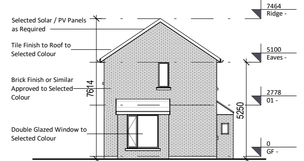
⑥ Gable Elevation Type B (Full Brick) 1 : 200
