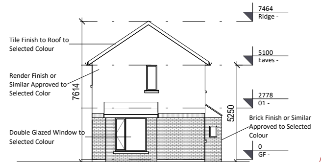
⑦ Gable Elevation Type B (Half Brick) 1 : 200
