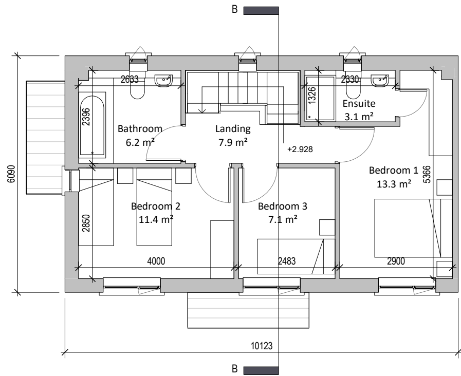
② First Floor Semi Detached with Bay Window 1 : 100
