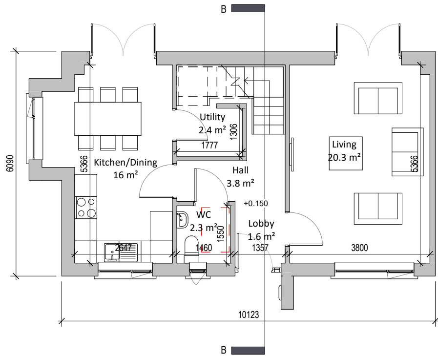
① Ground Floor Semi Detached with Bay Window 1 : 100
