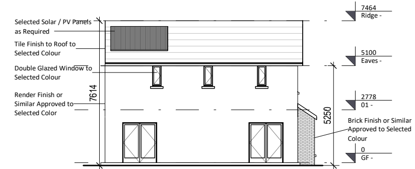
⑤ Rear Elevation Type B 1 : 200
